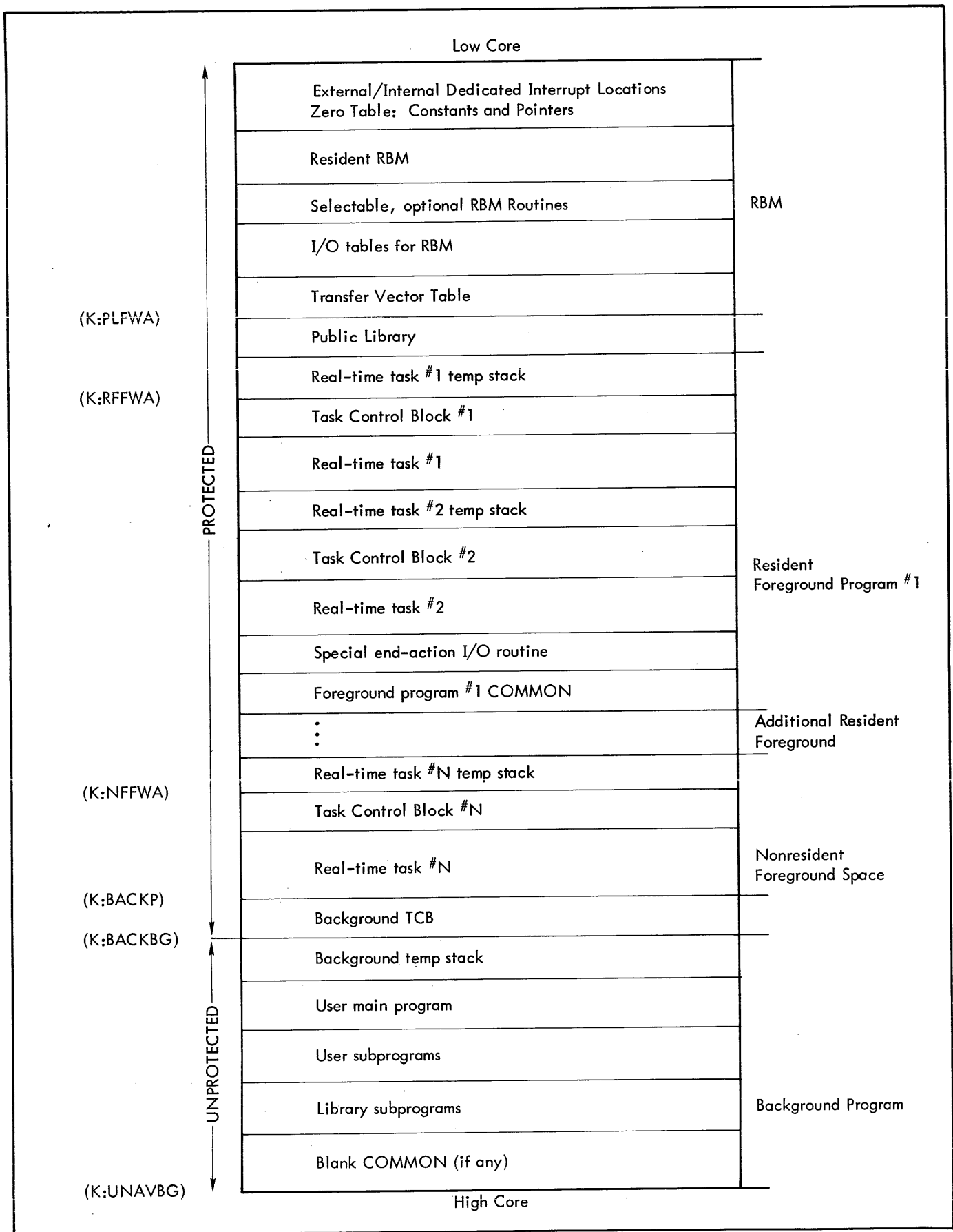
Figure 10. RBM Core Memory Allocation Example
